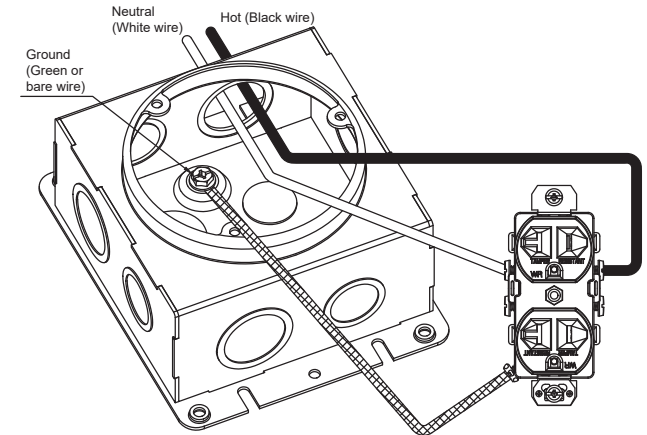
FB-02 junction box sold separately
